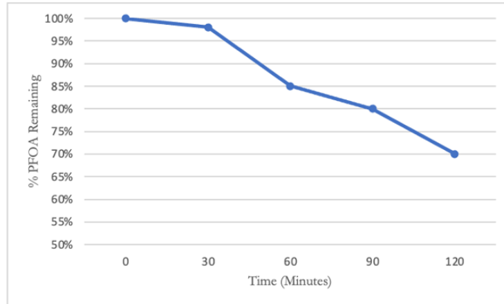
Graph1: PFOA Removed versus time, NO UV
