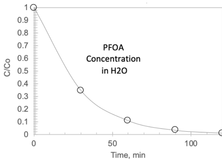
Graph 2: PFOA Removed versus time, WITH UV
